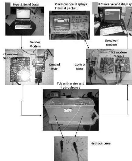
Figure 2: Hardware setup for demonstration of through-water data transmission.
